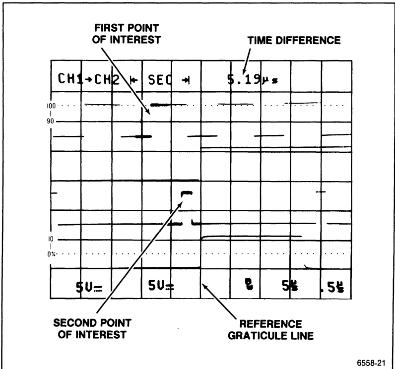
Figure 5-6. Time difference between two delays.
