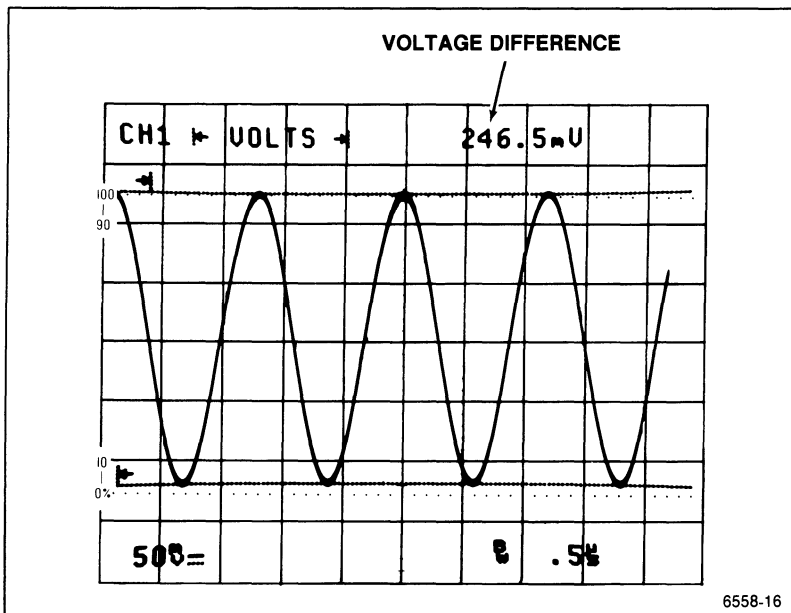
Figure 5-1. Voltage difference measurement using cursors.
