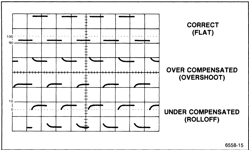
Figure 4-1. Probe compensation.
