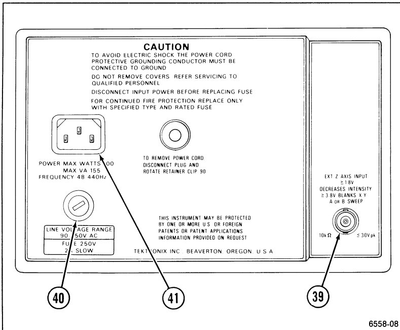
Figure 2-6. Rear panel connectors and fuse.
