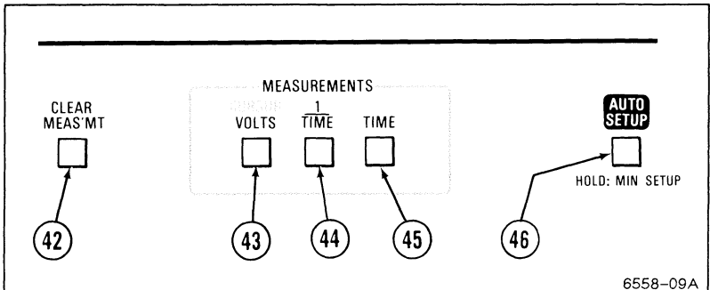
Figure 2-7. Measurement controls.
