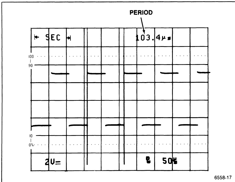
Figure 5-2. Period measurement.
