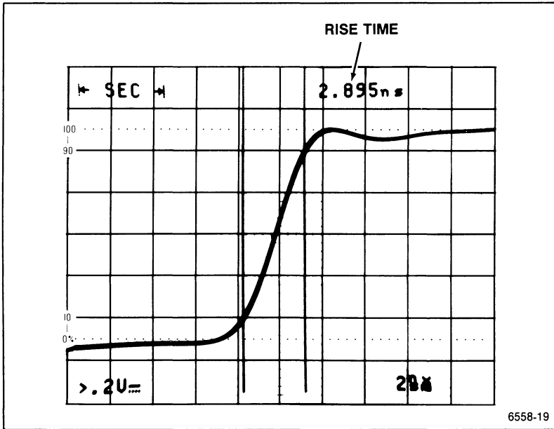
Figure 5-4. Rise-time measurement.
